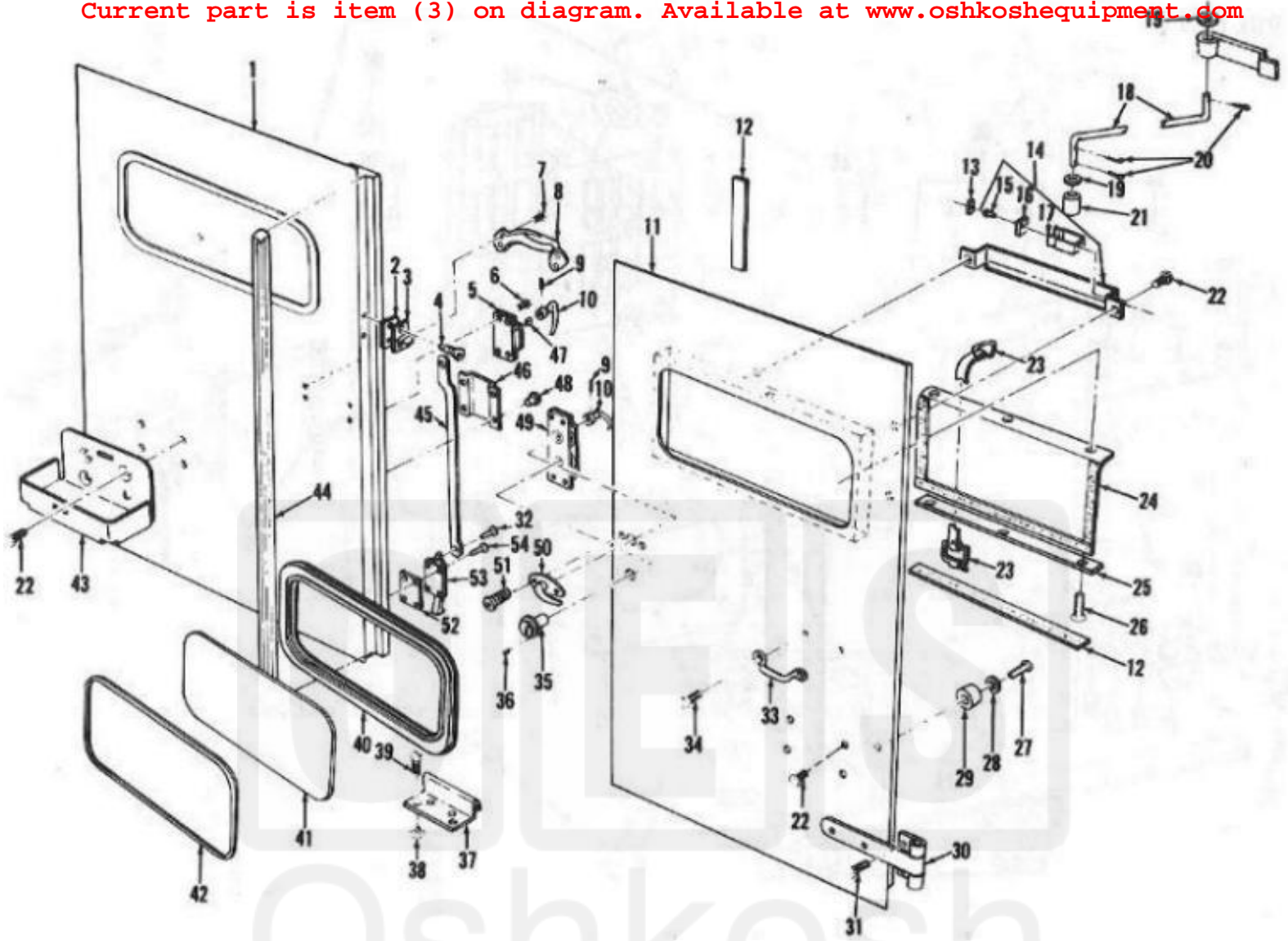
Figure 121: Ambulance Rear Doors and Related Parts Page 297
